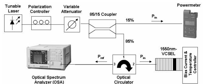
Fig. 1. Experimental set-up for orthogonal optical injection in a VCSEL.
