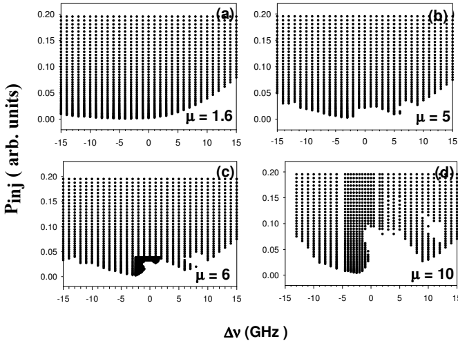
Fig. 6. Calculated injected optical power versus detuning ( P_{inj} - \Delta\nu plane). A black point indicates the occurrence of PS for (a) \mu=1.6 , (b) \mu=5 , (c) \mu=6 , (d) \mu=10 .
