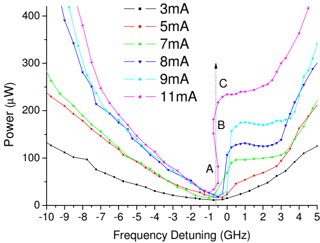
Fig. 3. (color online) Measured minimum injected power required for PS as a function of the frequency detuning for several values of the VCSEL current.
