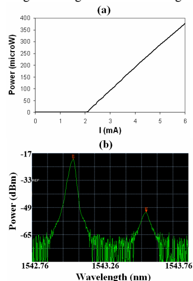
Fig. 2. (color online) (a) L-I Curve of the 1550nm-VCSEL. (b) Spectrum of the device biased with a current of 2.50 mA.
