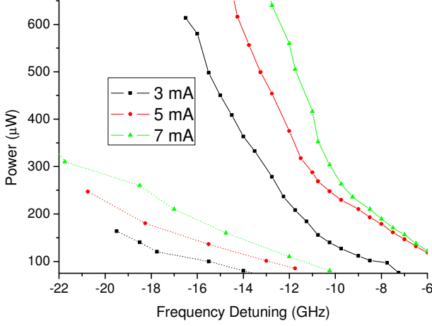
Fig. 4. (color online) Measured injected power required for PS as a function of the frequency detuning for several values of the VCSEL current. Results corresponding to increasing and decreasing the injected power are plotted with solid and dotted lines, respectively
