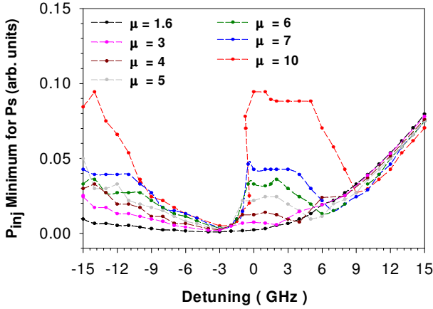
Fig. 5. (color online) Calculated minimum value of P_{inj} necessary to obtain PS as a function of the detuning \Delta\nu for different values of injected current, \mu
