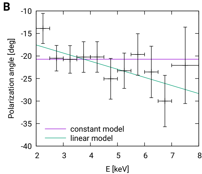
Figure S5: Energy dependence of the observed polarization degree (A) and polarization angle (B). The data (black crosses with 1\sigma error bars) are produced using the PCUBE algorithm of the xpbin tool and summed over all detector units. The constant (violet) and linear (green) models fitted to the data are also depicted (see the text for details).
