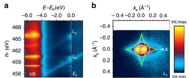
Figure 1 | Experimental low-temperature (12 K) overview SX-ARPES data. (a) Resonance (angle-integrated) photoemission intensity map, identifying the 2DES signal at the L_3 and L_2 resonances of the interface Ti ions. (b) FS map at the L_3 -resonance, where the superimposed theoretical FS contours identify the d_{xy} (pink) and d_{yz} (green) sheets. The colour bar indicates the intensity (Int.) maximum and minimum.
