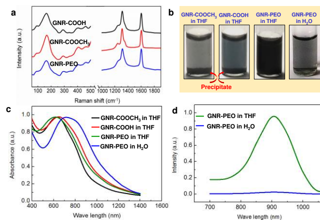
Figure 1. (a) Raman spectra of the GNRs with identical mean lengths of \sim 30 nm (excited at 638 nm). (b) Photos of GNR dispersions in THF (1.0 mg mL -1 for GNR backbone) and in H 2 O (0.2 mg mL -1 ) after sonication for 5 min. (c) UV-Vis spectra of GNR dispersions (0.01 mg mL -1 ). (d) PL spectra of GNR-PEO dispersions (0.01 mg mL -1 ).
