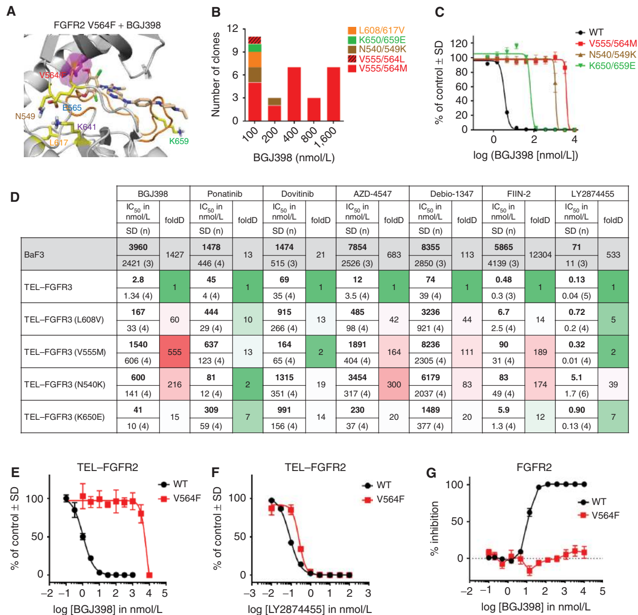
Figure 2. FGFR point mutations confer resistance to BGJ398 and other FGFR inhibitors. A , In silico model of BGJ398 in binding pocket of FGFR2 , demonstrating steric clash in the context of a V564F mutation. B and C , Mutagenesis screen in BaF3 cells that were engineered to express a TEL-FGFR3 fusion protein and subjected to increasing doses of BGJ398. The bar graph in B indicates the number of BGJ398-resistant clones isolated with indicated FGFR3 point mutations, with higher doses of BGJ398 resulting exclusively in colonies harboring the V555M gatekeeper mutation. Proliferation was quantified in C after 3 days with Alamar blue. Corresponding FGFR2 amino acids are indicated after the slash. D , IC 50 values for BaF3 cells expressing the indicated constructs and treated with a variety of inhibitors. E and F , Proliferation assays with BaF3 cells expressing the FGFR2 V564F constructs and treated with increasing doses of either BGJ398 ( E ) or LY287445 ( F ). G , Phospho-FGFR2 ELISA demonstrating that FGFR2 V564F is resistant to inhibition by BGJ398 compared with wild-type (WT).
