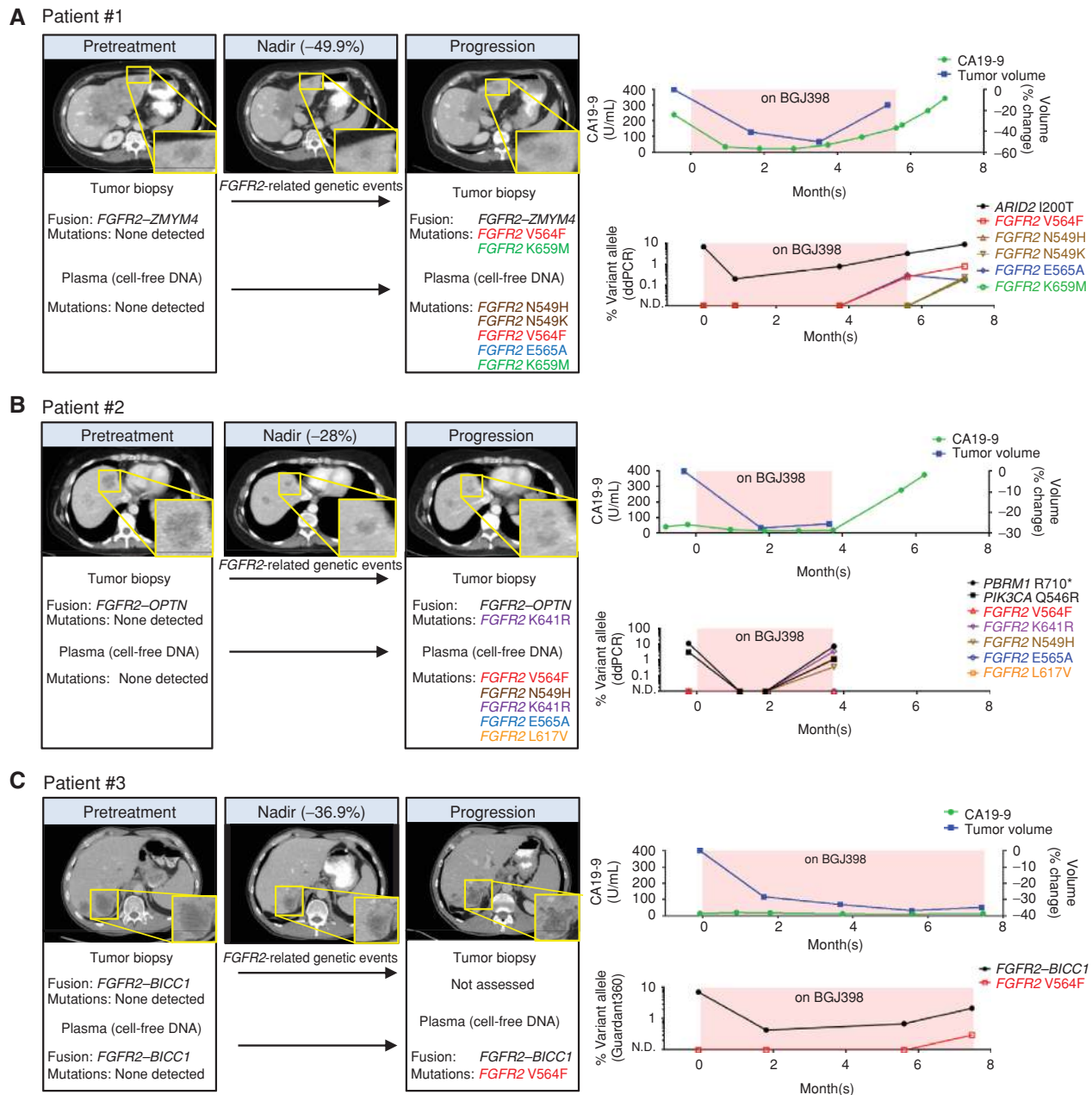
Figure 1. Clinical acquired resistance to BGJ398. A-C (left), Axial contrast-enhanced CT images in the portal venous phase demonstrating initial response lesions that subsequently progressed despite BGJ398 therapy. The inset shows higher magnification of responsive/resistant lesion. FGFR2 -related genetic events detected by SFA, RNA sequencing, WES, or the Guardant360 assay are documented in the text below CT images. Top right, graphs illustrating serial CA 19-9 serum levels and tumor volume measurements by RECIST v1.1 criteria for patients 1 to 3, respectively. The pink box indicates time while the patient was receiving BGJ398. Bottom right, percent allele burden in cfDNA of the indicated mutations from patient 1 ( A ), patient 2 ( B ), and patient 3 ( C ) were monitored over time with ddPCR. The pink box indicates time while the patient was receiving BGJ398. ddPCR, droplet digital PCR; N.D., not detected; WES, whole-exome sequencing.
