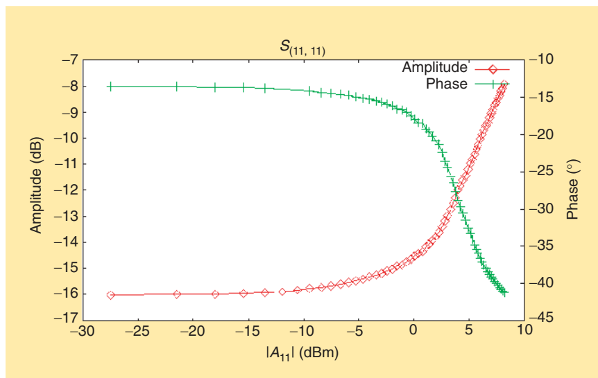
Figure 6. Large-signal reflection: S_{11,11}(\cdot) .
