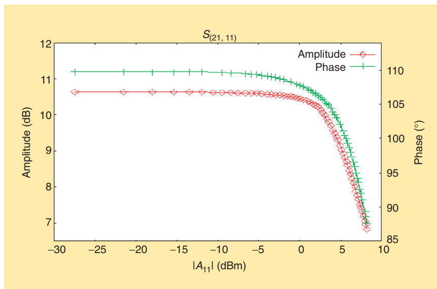
Figure 5. Compression and AM-PM: S_{21,11}(\cdot) .
