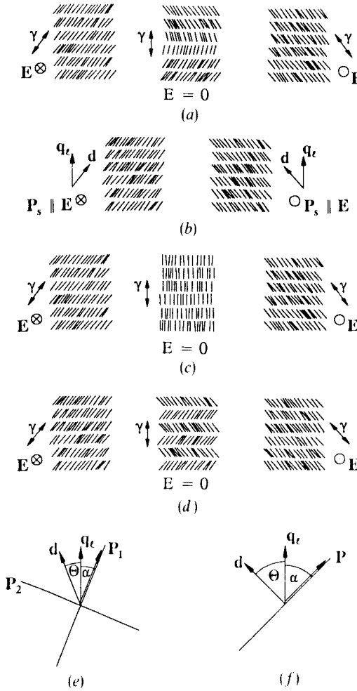
Figure 11. (a-d) Director fields for different switching effects in ferroelectric liquid crystals ( \gamma : optical axis, q_i : layer normal, d : director, P_s : spontaneous polarization). (a) Helical unwinding. (b) bistable switching in surface-stabilized FLC displays. (c) electroclinic effect. (d) tri-stable switching in antiferroelectric liquid crystals. (e-f) azimuthal orientation of the layer normal q_i with respect to the polarizer P_1 and analyser P_2 , in order to maximize the contrast when (e) the optical retardation of the PDLC film, or (f) the scattering effect due to matching or mismatching of the refractive indices is used.
