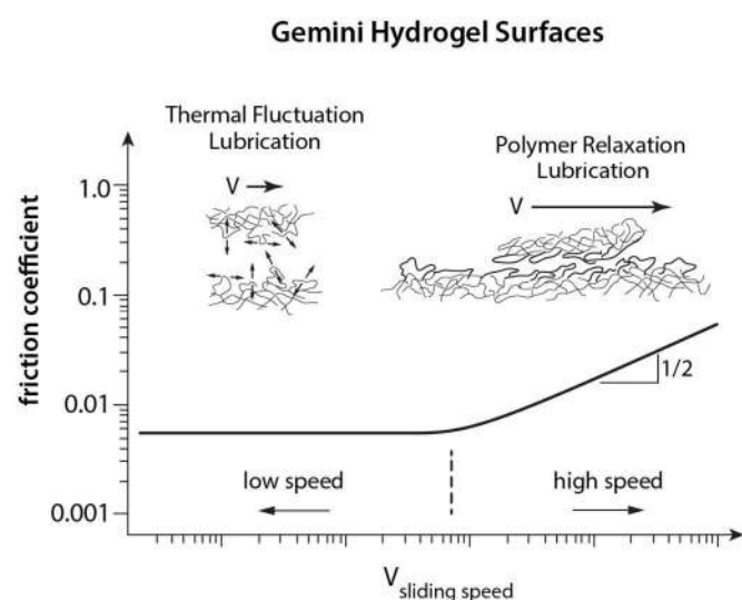
Fig. 5 Gemini hydrogel lubrication model. For low speeds, thermal fluctuation lubrication dominates and the coefficient of friction remains low. For high speeds, polymer relaxation and adhesion are the dominating mechanisms and a corresponding increase of friction coefficient to the 1/2 power arises.
