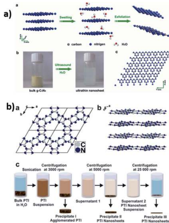
Fig. 17 (a) Scheme of the synthesis of dispersed CN nanosheets by liquid-phase exfoliation (a swelling step, followed by exfoliation using ultrasonication as an external mechanical force). Reproduced from ref. 591, copyright (2012) American Chemical Society. (b) Scheme of the preparation of ultrathin PTI materials by sequential exfoliation. Reproduced from ref. 613, copyright (2014) American Chemical Society.
