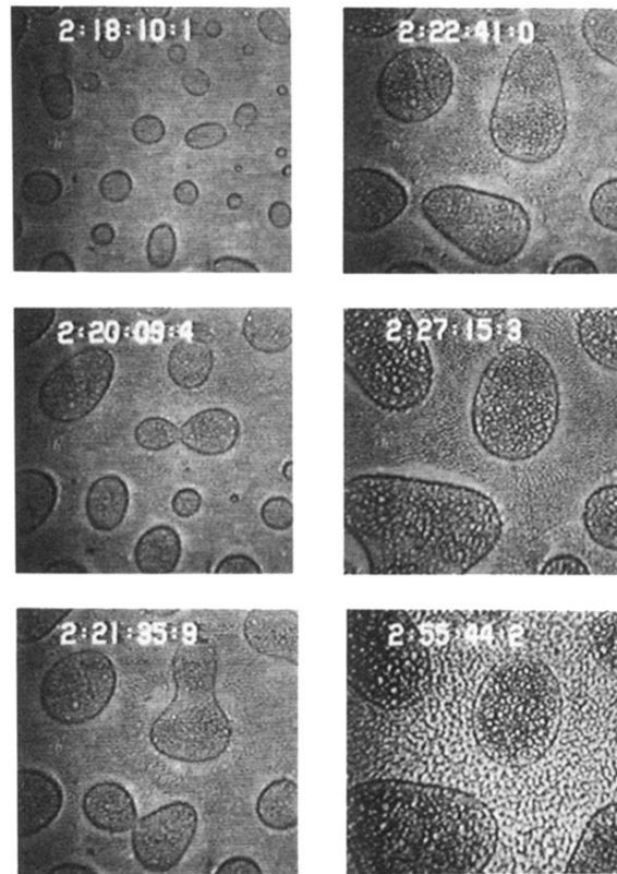
FIG. 5. Micrographs of the cascade phenomena where phase separation occurs for a second time. The horizontal dimension of each micrograph is 180 \mu\text{m} .
