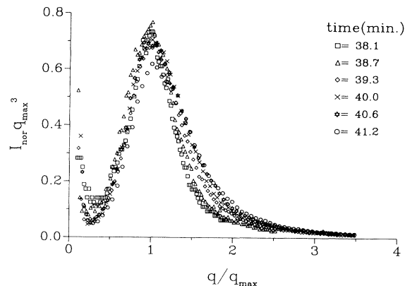
FIG. 2. The scaling function F(q/q_{\max}) = I_{\text{nor}} q_{\max}^3 vs the scaled wave vector q/q_{\max} .
