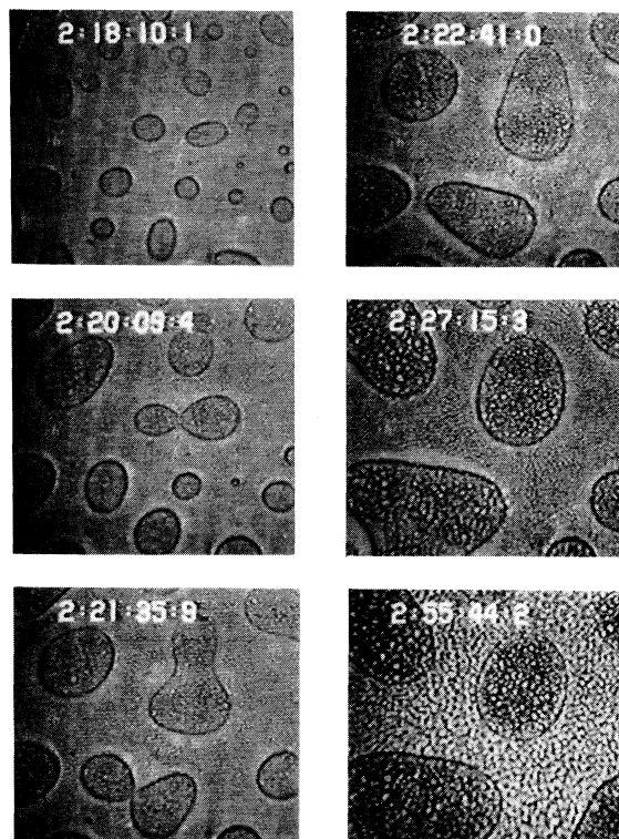
FIG. 5. Micrographs of the cascade phenomena where phase separation occurs for a second time. The horizontal dimension of each micrograph is 180 \mu\text{m} .
