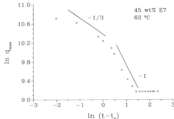
FIG. 3. \ln q_{\max} vs \ln(t - t_0) . The slope is \alpha .
