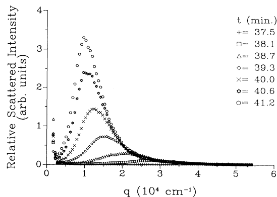
FIG. 1. Scattered intensity I(q,t) vs the scattering vector q .
