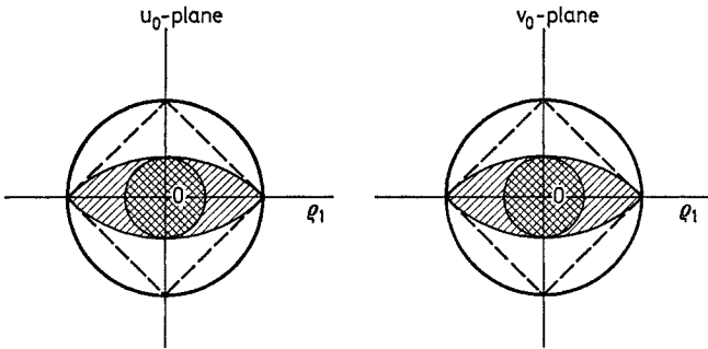
Fig. 2. The domain of analyticity of \Psi in \pi_0 contains the topological product of the shaded domains
