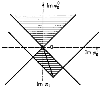
Fig. 1. Tubes of analyticity in \pi_0 for fixed \pi_1 \in V^- and \pi_1 + \pi_2 \in V^+
