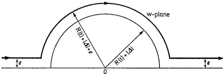
Fig. 3. The contour \mathcal{C}(\varepsilon)
