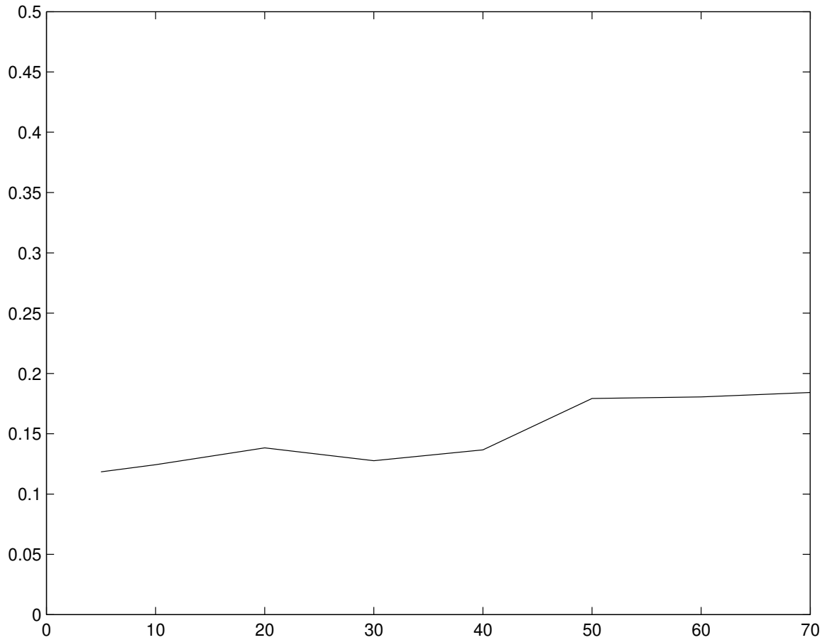
Figure 9. Normalized numerical cost for the construction of the stochastic preconditioner as a function of its bandwidth \ell : graph of \ell \mapsto \text{eff}_1(\ell) ; N_1 = 4,500 , N'_1 = 1 ; N_2 = 1,800 ; P_1 = 2 , P'_1 = 0 ; P_2 = 4 .
