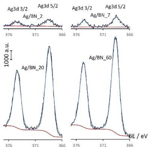
Figure 2: XPS spectra of AgNPs.
