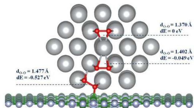
Figure 8. Oxygen molecule positions on h -BN/AgNP. The Ag, B, N, O atoms are marked as large grey, small green, small grey and red balls respectively.
