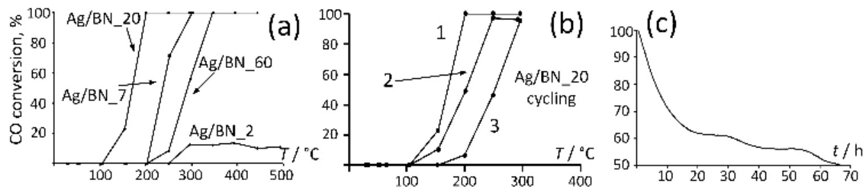
Figure 3: (a) Catalytic activity of all samples; (b) catalytic cycling Ag/BN_20; (c) catalytic stability Ag/BN_20.
