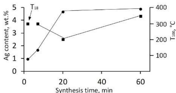
Figure 4: Correlation between Ag content, synthesis time and temperature of CO conversion. ■ - T_{100} , (For Ag/BN_2 sample T_{18} is given); ● - Ag content.
