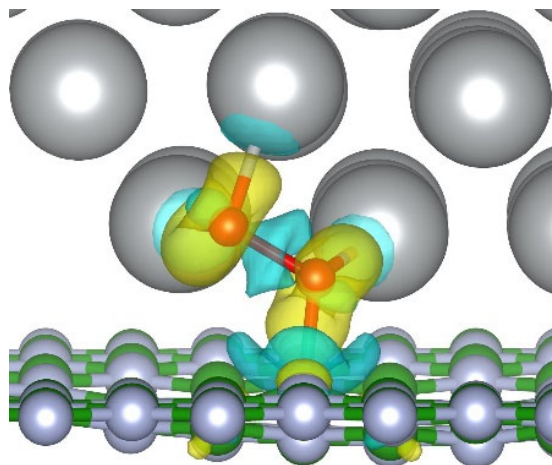
Figure 9. Charge difference between O 2 and h -BN/AgNP. The iso-surface level is equal to 0.005e/Å. The electron excess and deficiency regions are marked by yellow and cyan colours. The Ag, B, N, O atoms marked as big grey, small green, small grey and red balls, respectively.
