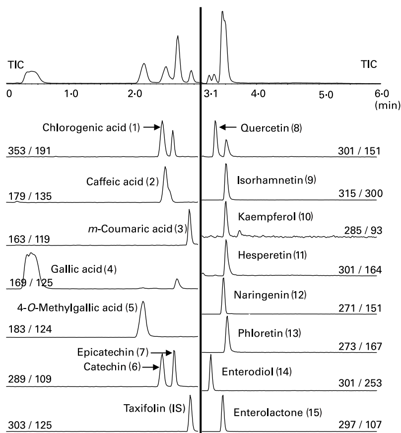
Fig. 2. Total ion chromatogram (TIC) and extracted single ion chromatograms of a mixture of fifteen dietary polyphenols (10 \mu M) obtained by an HPLC-electrospray-tandem mass spectrometry method in multiple reaction monitoring mode with negative ionisation. IS, internal standard.
