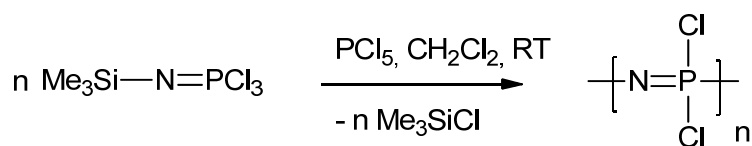
Figure 4. The living cationic polymerization route to polydichlorophosphazene.
