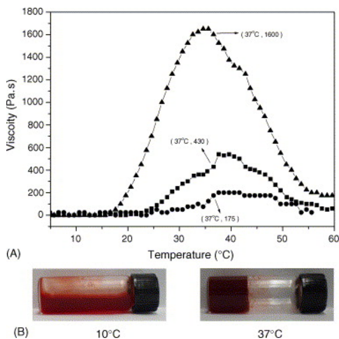
Figure 13. (a) Change of viscosity with temperature of polyphosphazenes cosubstituted with mPEG ( M_n = 550 ) and isoleucine ethyl ester and glycyl lactate ethyl ester groups at polymer concentrations of 7 wt. % (●), 10 wt. % (■), and 15 wt. % (▲). (b) Reversible gelation behavior is observed at temperatures between 10 and 37 °C. Reprinted from [121]), with permission from Elsevier.
