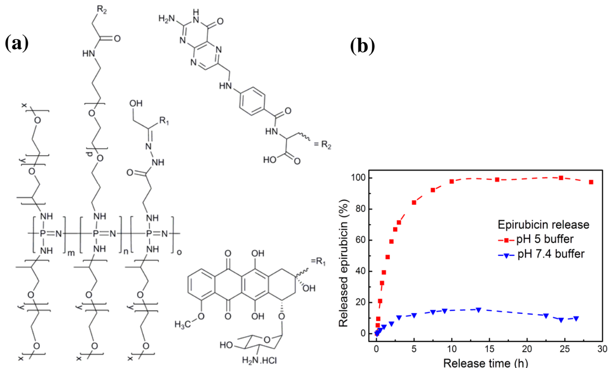
Figure 11. (a) Water soluble polyphosphazene loaded with a folic acid targeting ligands and epirubicin via a pH labile hydrazone bond. (b) Release of epirubicin from the hydrazone-linked polyphosphazene pH 5 (■) and pH 7.4 (▼). Originally published in [29] and reproduced by permission of The Royal Society of Chemistry.
