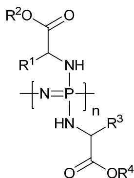
Figure 7. Generic structure for amino acid ester substituted poly[(organo)phosphazenes]. R_1 – R_4 can be varied to give a range of poly[(organo)phosphazenes] with tailored degradation rates.
