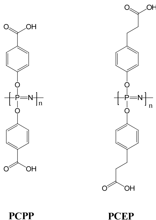
Figure 15. The most important polyphosphazenes most used as a basis for vaccine delivery vehicles are the sodium salts of poly[bis(carboxyphenoxy)phosphazene] PCPP and poly[bis(carboxyethylphenoxy)phosphazene] PCEP.
