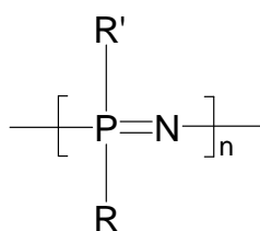
Figure 2. Some examples of poly[(organo)phosphazenes] with varied properties. ( T_g values as reported in [25]).
