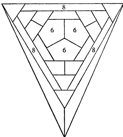
FIGURE 3 (DUE TO W. T. TUTTE)
