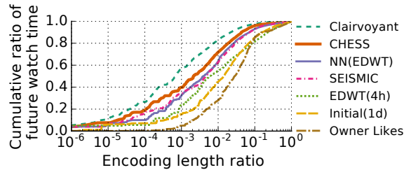
Figure 5: Single prediction results shown by the cumulative ratio of future watch time of the videos selected by each predictor for a given encoding length ratio.
