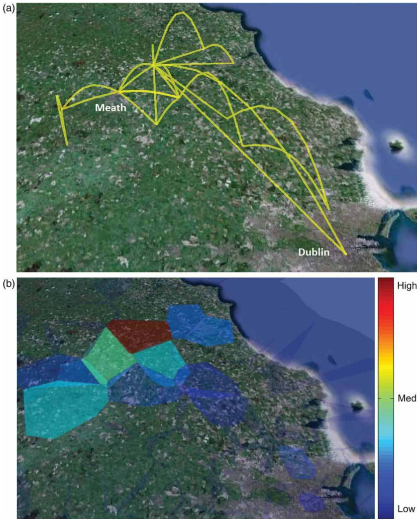
Figure 8: Visualization of an example: (a) subscriber transition probability matrix, Q_{ij} , where heights correspond to transition intensity; (b) corresponding fixed row vector, w_{ij} , where polygon color corresponds to state weight.
