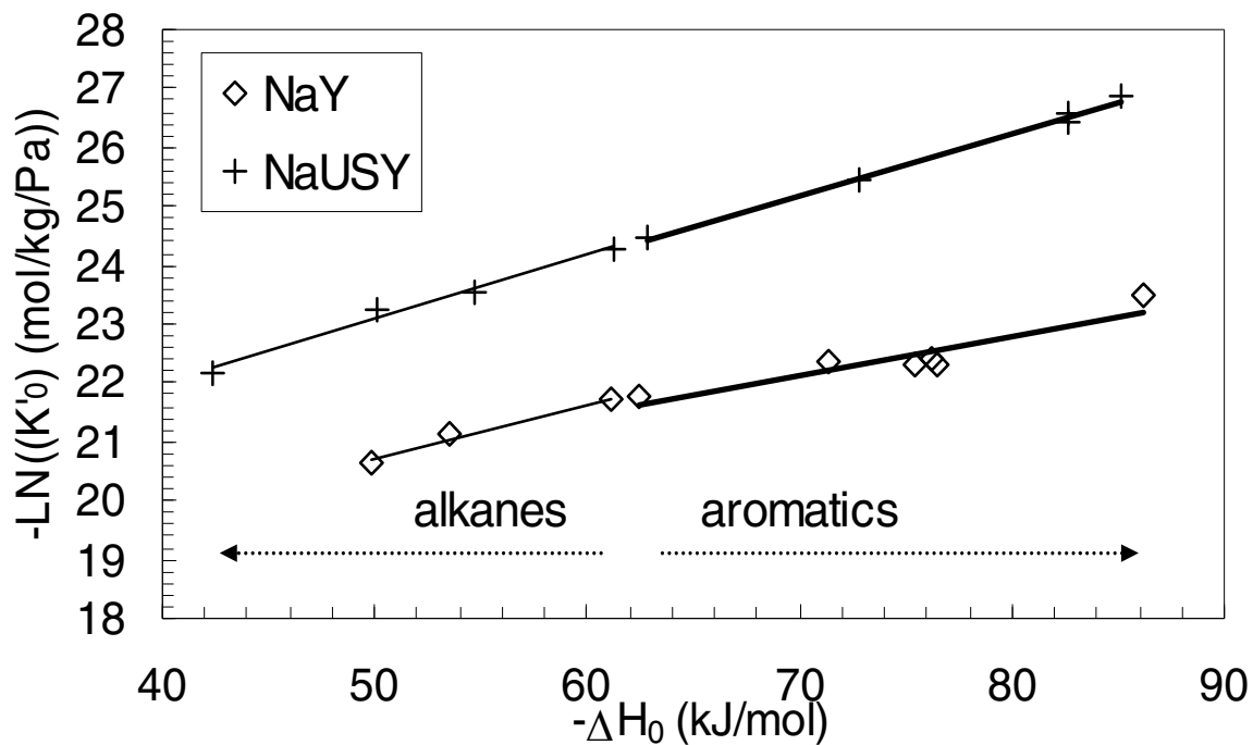
Figure S1: Compensation plot of n -alkanes and aromatics on NaY and NaUSY [PhD dissertation Inge Daems, Vrije Universiteit Brussel, Belgium, december 2005, pp. 49.].
