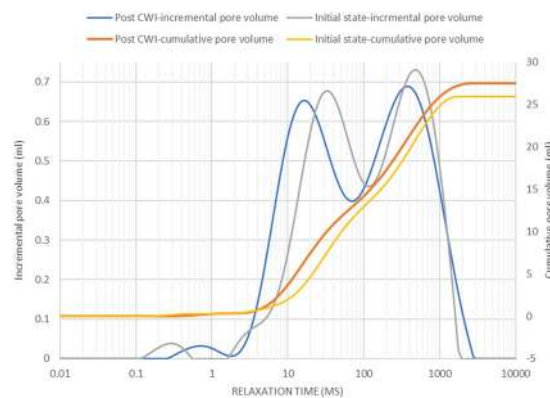
Figure 7. T_2 relaxation time profiles of Core A before and after carbonated brine injection (CWI) step indicates the changes in pore size populations.
