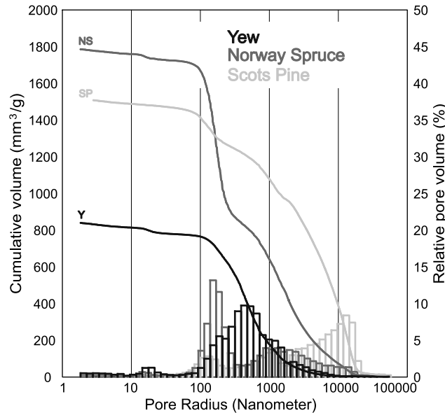
Fig. 8 Cumulative pore volume and histogram of relative pore volume as a function of the pore radius of Yew, European spruce and Scots pine, illustrating the different distribution types of softwood
