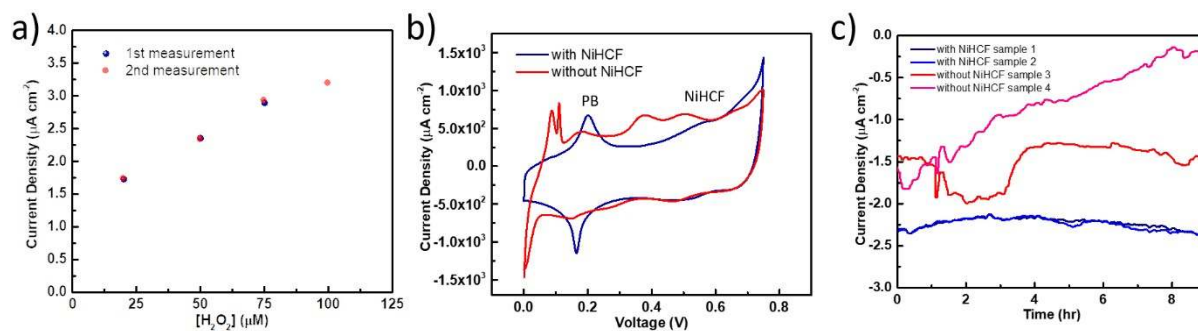
Figure S4. a) Sensitivity of nanotextured PB-based \text{H}_2\text{O}_2 sensor with NiHCF layer. b) CV curves of glucose sensors with/without NiHCF layer after 20 hours long time measurements. c) 9 hours long-term amperometric response of glucose sensors with/without NiHCF layer in 50 \mu\text{M} glucose electrolyte.
