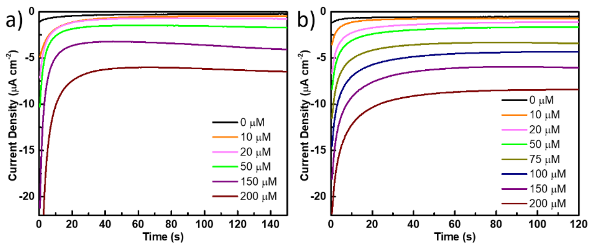
Figure S6. Amperometric responses of nanotextured glucose sensors with a) agarose and b) chitosan bulk membranes.
