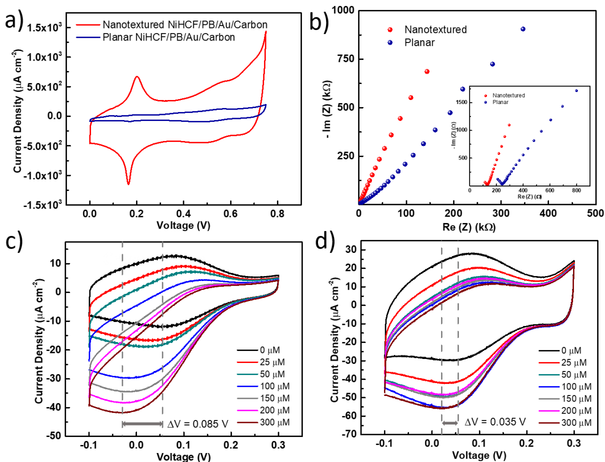
Figure S5. a) CV curves of planar and nanotextured glucose sensors in supporting solutions. b) EIS measurements of planar and nanotextured sensor electrodes. CV curves of c) planar and d) nanotextured glucose sensors with delaminated enzymatic membranes in different concentrations of glucose/PBS buffer solutions at the scan rate of 100 \text{mV s}^{-1} .
