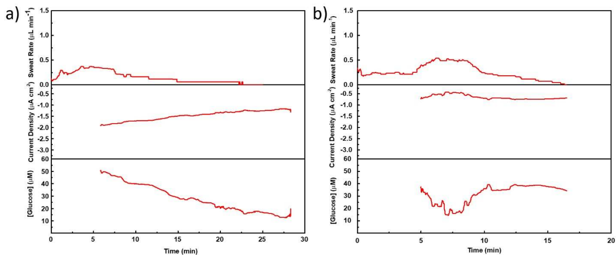
Figure S8. a-b) Sweat rates, amperometric responses and measured sweat glucose concentrations during on-body iontophoresis measurements on different subjects.
