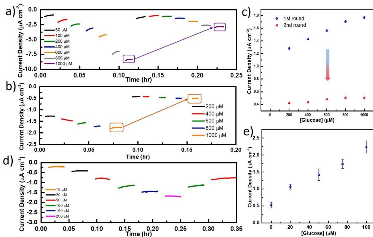
Figure S3. Cyclic amperometric response of conventional glucose sensors based on a) Au/PB/bulk agarose enzymatic membrane, b) printed carbon/PB/bulk agarose enzymatic membrane and c) its decreased sensitivity. d) Cyclic amperometric response of glucose sensors based on printed carbon /PB/porous enzymatic membrane and e) its reproducibility.
