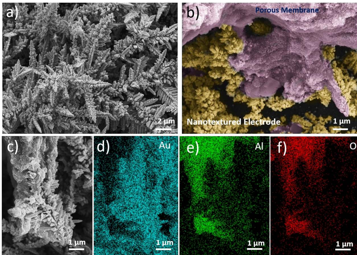
Figure S1. SEM images a) nanotextured NiHCF/PB/Au electrode and b) Porous membrane anchored with nanotextured electrode. c-f) EDS images of porous membrane anchored to the nanotextured electrode.
