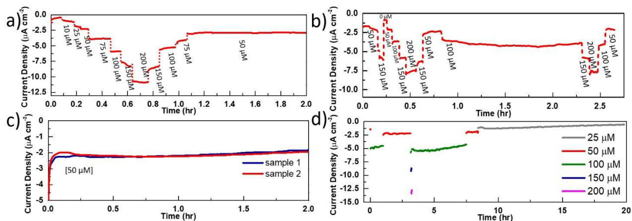
Figure S7. Amperometric responses of nanotextured glucose sensors with porous enzymatic membranes in the glucose solutions a-b) with dynamically tuned or c) constant concentrations. d) Repeated result on long-term amperometric response.
