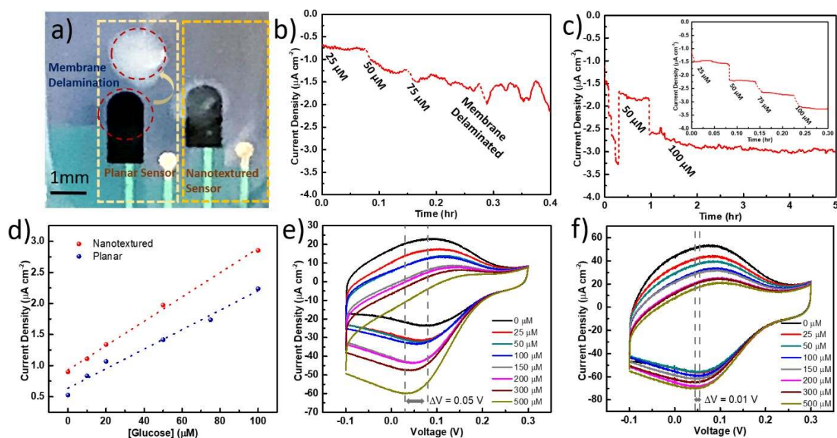
Figure 3. Performance enhancement of nanostructured glucose sensors with porous enzymatic membranes. a) Photos showing delamination of porous enzymatic membrane from planar electrode (left) after 1 hour measurement and enhanced adhesion to nanotextured electrode (right). Amperometric response of b) planar glucose sensors with membrane delamination occurs during measurements and c) nanotextured glucose sensors without membrane delamination (inset: focused amperometric response in the first 20 mins). d) Sensitivities of planar and nanotextured glucose sensors. CV curves of e) planar and f) nanotextured glucose sensors in different concentrations of glucose/PBS buffer solutions at the scan rate of 100 \text{ mV s}^{-1} .
