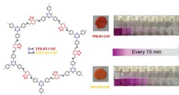
Fig. 16 Structures of BT-COFs and pictures of the corresponding powder and photographs of the photocatalytic reduction using TPB-BT-COF and TAPT-BT-COF. Reproduced from ref. 140 with permission from the Royal Society of Chemistry, Copyright 2019.
