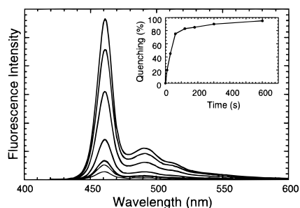
Figure 2. The time-dependent fluorescence intensity of 2 ( 25 \pm 5 \text{ \AA} thickness) upon exposure to TNT vapor (room temperature) at 0, 10, 30, 60, 120, 180, 300, and 600 s (top to bottom) and the fluorescence quenching (%) against time (inset).
