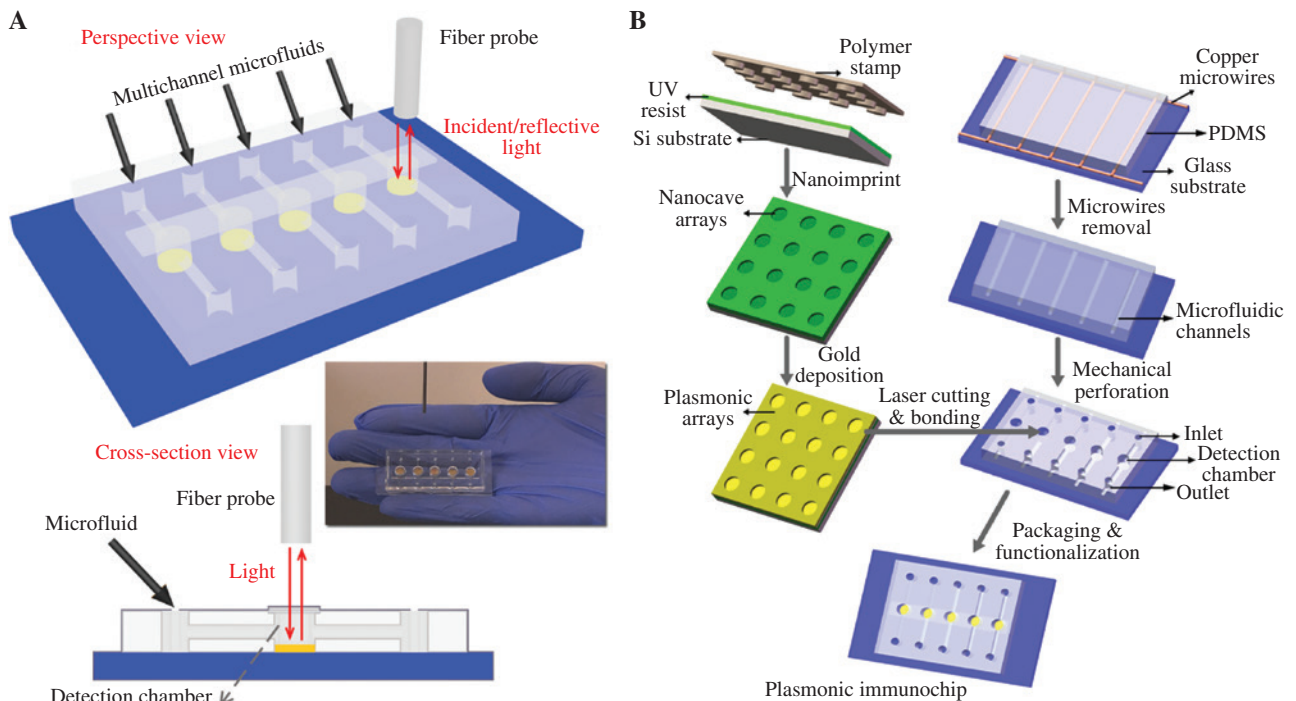
Figure 1: Sensing configuration and biochip fabrication.
