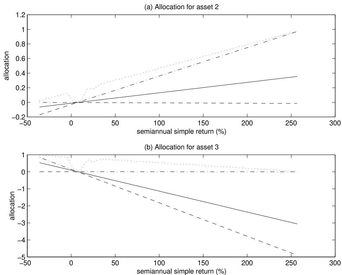
Figure 3-11: Weights of an optimal portfolio. Put-Call data. (no risk-free asset, shortsals allowed)
