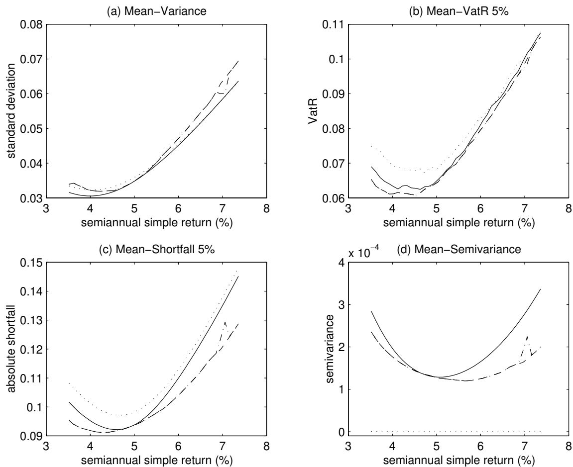
Figure 3-5: Efficient frontiers. Option-based strategies data. (no risk-free asset, shortsales allowed)
