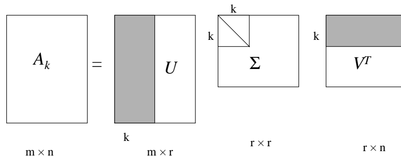
Figure 3 – Singular value decomposition
