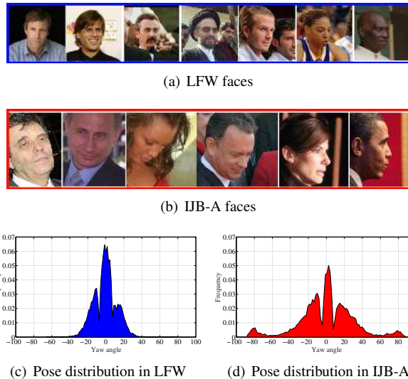
Figure 1: Top : images with increasing yaw angle from left to right in LFW (blue) and IJB-A (red). Bottom : Pose distributions (yaw angle) in the two datasets.
