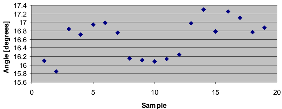
Figure 7. Repeatability test for 20 successive measurements. Object rotated about x axis with an angle of 16 degree. Resulting mean value 16.64^\circ , standard deviation 0.44.
