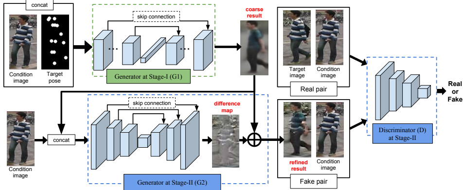
Figure 2: The overall framework of our Pose Guided Person Generation Network ( PG^2 ). It contains two stages. Stage-I focuses on pose integration and generates an initial result that captures the global structure of the human. Stage-II focuses on refining the initial result via adversarial training and generates sharper images.
