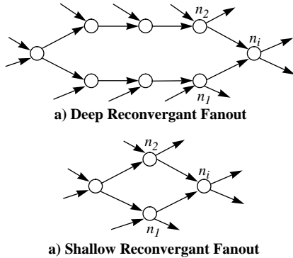
Figure 4: Reconvergent Fanout Regions
