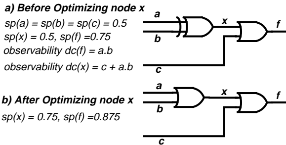
Figure 5: Effect of optimizations on signal probabilities
