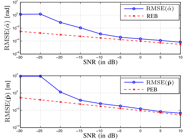
Fig. 8. RMSE in dB scale for the NLOS plotted against received SNR for rotation angle (top) and position (bottom) in the presence of a scatterer located at \mathbf{s}_k [m] = [1.5, 0.4]^T . The red lines show the corresponding bounds.
