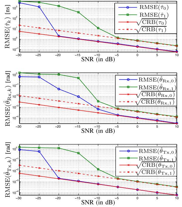
Fig. 7. RMSE in dB scale for the NLOS plotted against received SNR for TOA and AOA/AOD in the presence of a scatterer located at \mathbf{s}_k [m] = [1.5, 0.4]^T . The red lines show the corresponding bounds.
