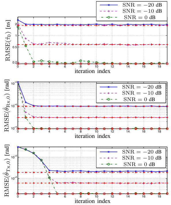
Fig. 3. The evolution of RMSE of TOA and AOA/AOD for the LOS for SNR = -20 dB, -10 dB, 0 dB. The red lines with the same markers show the bounds for the same value of SNR corresponding to the RMSE of TOA and AOA/AOD.
