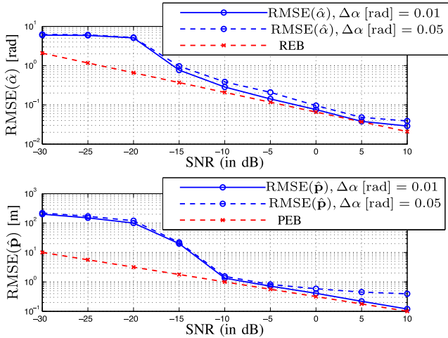
Fig. 9. RMSE in dB scale plotted against received SNR for rotation angle (top) and position (bottom) in the OLOS with three scatterers located at \mathbf{s}_k [m] = [1.5, 0.4 + 0.5(k-1)]^T for k = 1, 2, 3 and \Delta\alpha [rad] = \{0.01, 0.05\} . The red lines show the corresponding bounds.
