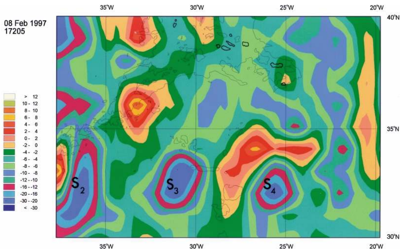
Figure 13. Altimeter sea level anomalies (cm scale in colour) corresponding to Figure 12. S_3 and S_4 (labelled) are evident near 31°W and 26°W (~32.5°N). Orange region to the north of S_4 matches the warm water region W in Figure 12 and blue meridional patch near 23°W corresponds to the cold streaks marked c.
