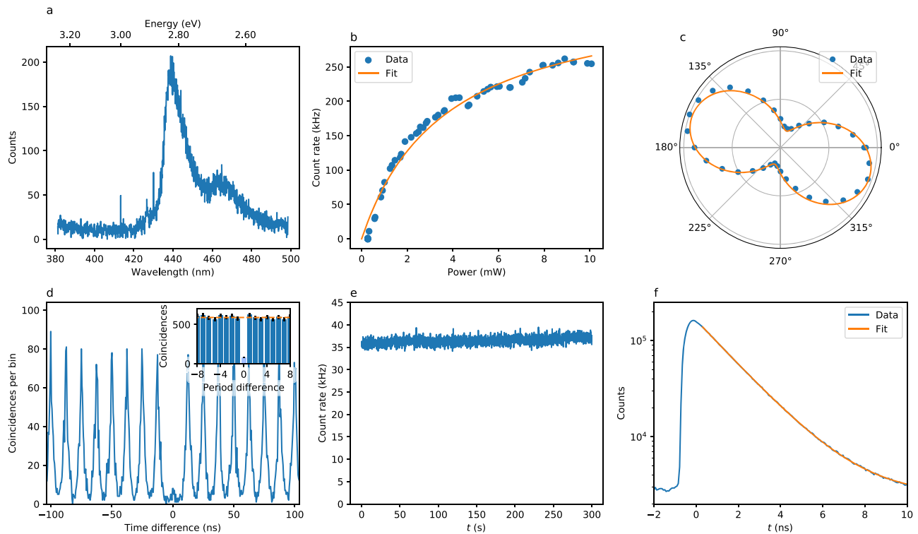
Fig. 2 Photophysical characterization of an individual SPE at room temperature. a Emission spectrum of \text{SPE}_1 , showing a main peak centred at 440 nm (ZPL) and a phonon replica at 465 nm. b Count rate as a function of the laser power in cw regime. The orange curve is a fit to the data, from which we extract a saturation power of 3.7 mW and a maximum photon detection rate of 3.6 \times 10^5 \text{ Hz} . c Count rate as a function of the angle of a polarizer placed before the detector, showing linearly polarized emission. The orange curve is a sine fit of the data. d Photon correlations in pulsed regime measured with 315 \mu\text{W} excitation power and 80 MHz repetition rate, yielding g^{(2)}(0) = 0.12 \pm 0.01 and thus demonstrating single photon emission. Inset: period-wise integrated coincidences (error bars: 1 standard deviation). The dashed orange line denotes the classical limit. e Time trace of the photon detection rate with 100 ms binning, calculated from the same raw data as (d) . f Fluorescence decay in logarithmic scale, extracted from the same raw data as (d) . The orange curve is an exponential fit to the data, yielding \tau = 1.85 \text{ ns} .
