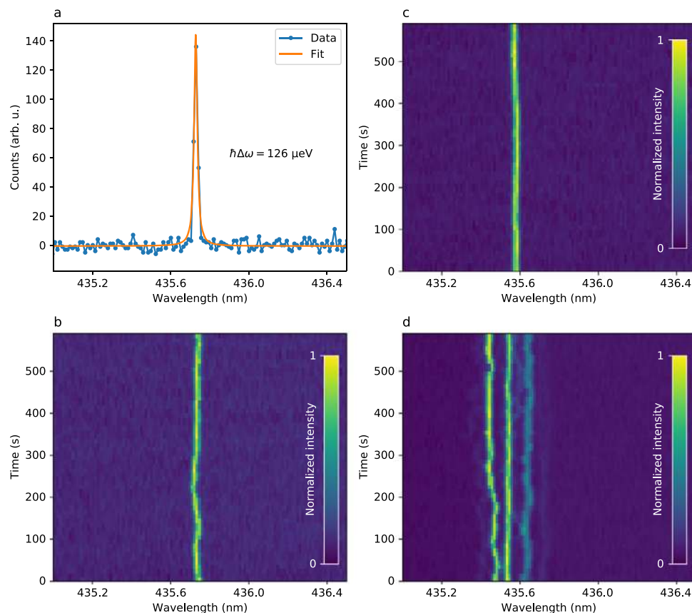
Fig. 4 Spectral properties of individual SPEs at low temperature (5 K). a High-resolution spectrum of SPE 1 ZPL, showing a resolution-limited line at 435.73 nm. b Spectral diffusion of SPE 1 ZPL during 600 s. The standard deviation of the centre wavelength over time is found to be 45 \mu\text{eV} , as determined by Lorentzian fits of the data. c Spectral diffusion of another SPE (SPE 2 ) and d spectral diffusion of an ensemble of three SPEs, with uncorrelated fluctuations of different magnitudes. All SPEs are excited with 1 mW cw laser light at 405 nm.
