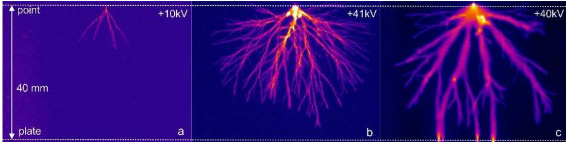
Figure 6. Typical photographs of positive streamers for parameter values indicated by A, B, C in figure 5. Panels a and b are made with the slow C 2 -supply, panel c with the fast C 1 -supply. The maximal voltage is a) +10 kV, b) +41 kV, and c) +40 kV. The white dotted lines indicate the electrode positions as in Figs. 2 and 4. The streamers in panel a at 10 kV have reached their maximal length; the streamers in panels b and c at \approx 40 kV are still propagating. Panels b and c demonstrate how strongly positive streamers at a voltage saturation value of 40 kV depend on the voltage rise time of the supply, as discussed in [32].
