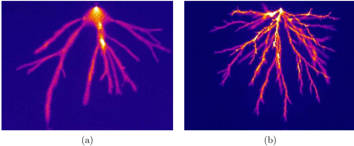
Figure 3. Streamers in a 4 cm gap at 0.4 bar (i.e., for p \cdot d_{gap} = 16 \text{ mm}\cdot\text{bar} ) and at 16 kV in a) air and b) \text{N}_2 . In these photos, the streamers are not seen to reach the cathode because the shutter of the camera is closed before that happens.
