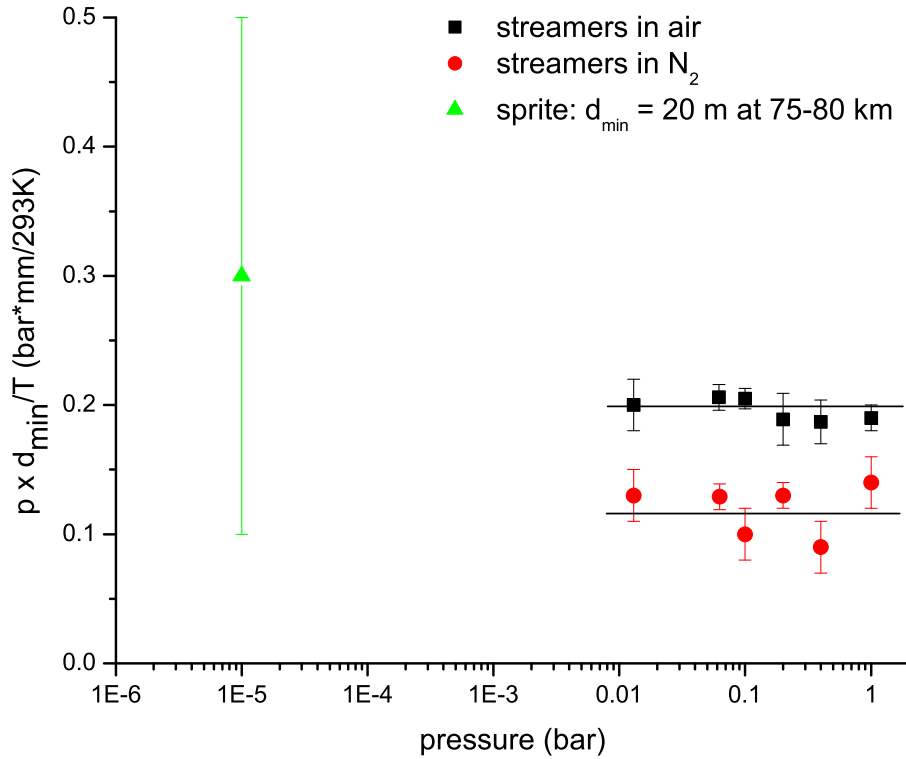
Figure 5. Reduced minimal streamer diameter d_{min} \cdot p/T as a function of pressure p ; here T is temperature and 293 K is room temperature. Black squares: experimental results in air. Red dots: Experimental results in our N_2 . Green triangle: minimal sprite diameter at 80 km height from [20].
