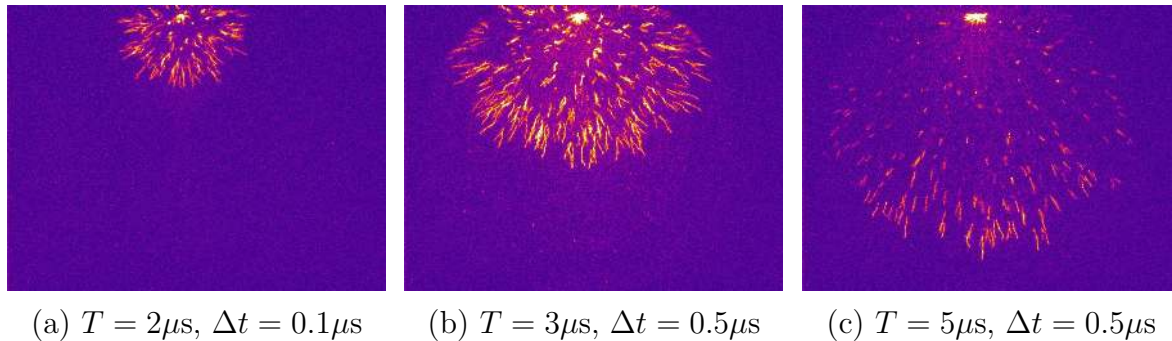
Figure 7. Time resolved photographs of streamers in a 16 cm gap in our \text{N}_2 at 1 bar at a voltage of 49 kV ( p \cdot d_{\text{gap}} = 160 \text{ mm}\cdot\text{bar} ). The gate delay T and exposure time \Delta t are indicated in each panel. The streamers reach the plate electrode some time after the exposure of panel (c). When the same experiment is performed in air at 1 bar, the streamers do not cross the gap.
