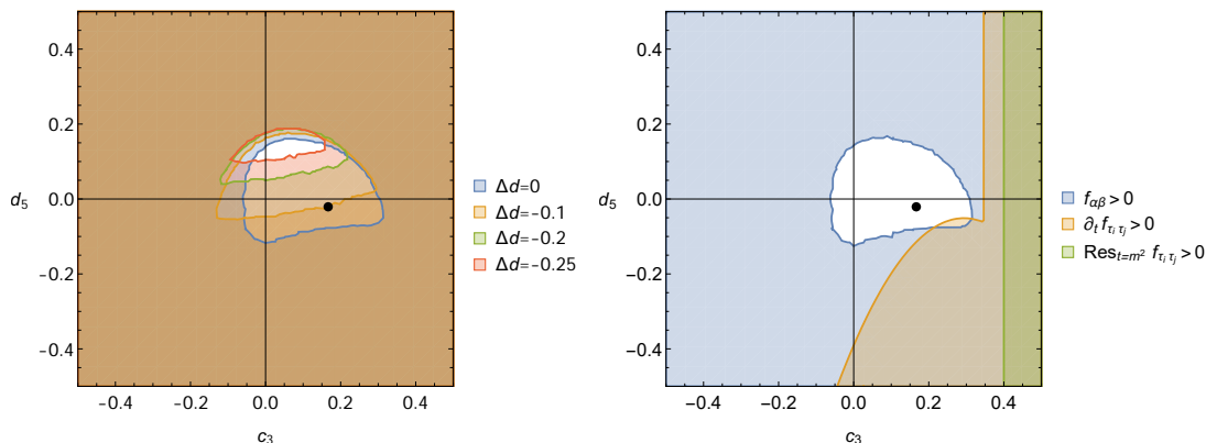
Figure 2. Parameter space of massive gravity constrained by analyticity. The forward limit bounds on \Lambda_5 massive gravity (left) gradually constricts as \Delta d is made more negative. However, going beyond the forward limit (6.34) rules out \Delta d \neq 0 completely. In \Lambda_3 massive gravity (right), the higher t derivative bounds marginally restrict the forward limit bounds. This lends further evidence to the idea that \Lambda_3 massive gravity may admit a Wilsonian UV completion within this narrow island.
