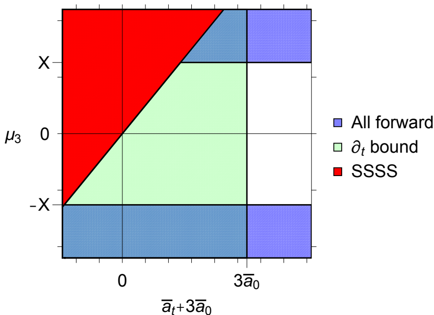
Figure 1. Parameter space for charged Galileon theory constrained by analyticity. A suppressed a_0 \sim m^2/\Lambda_\phi^2 is required to recover a Galileon symmetry in the decoupling limit. The forward limit bound from scattering four scalar modes was previously found in [7], which excluded the red region. By looking at scattering superpositions of modes, one use forward limit bounds to further restrict the parameter space to a semi-infinite strip (the white region plus the light green region) in the parameter space spanned by (\mu_3, \bar{a}_t + 3\bar{a}_0) . Utilizing the first \partial_t bound (i.e., going away from the limited forward limit formalism), we reduce this semi-infinite strip even further, potentially greatly, depending on the sign of 3\bar{a}_0 = 3a_0 - a_5 - C_1 - 4C_2 . In terms of the EFT coefficients in (3.5), we have 2\bar{a}_t = a_3 + a_4 - 2a_5 , \mu_3 = a_4 - a_5 - a_3/2 - C_1/2 - 2C_2 . The SSSS bound corresponds to \bar{a}_t + 3\bar{a}_0 - 2\mu_3 > 0 .
