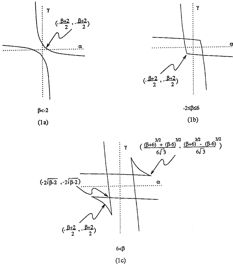
FIG. 1. Parametric curves from (4).
