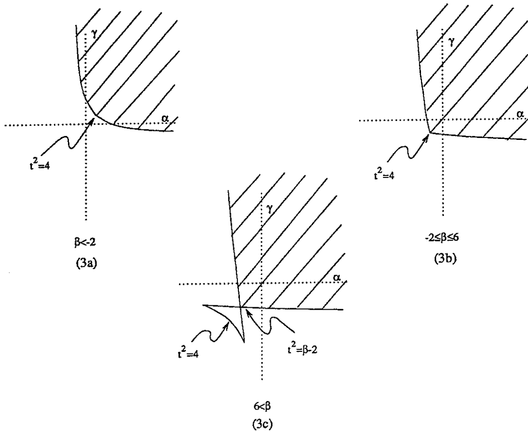
FIG. 3. Regions of positivity for the quartic polynomial.
