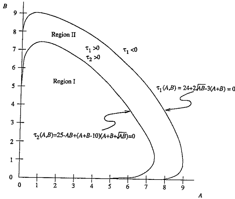
FIG. 6. Boundary regions on \eta(A, B) .
