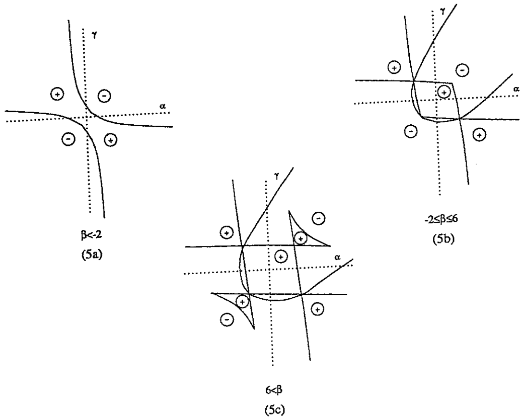
FIG. 5. Positivity conditions for the quartic polynomial.
