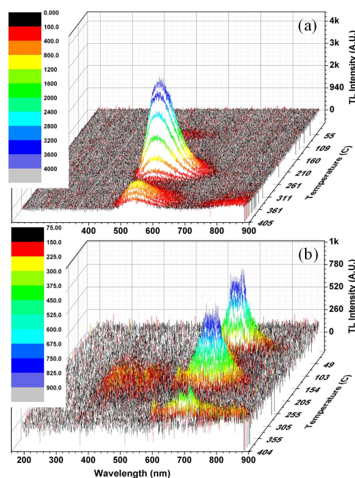
Fig. 1. TL spectra as a function of temperature and wavelength demonstrating the interaction between trapping defects and luminescence centers in single crystals of (a) Ce doped YAG, (b) undoped YAG.
