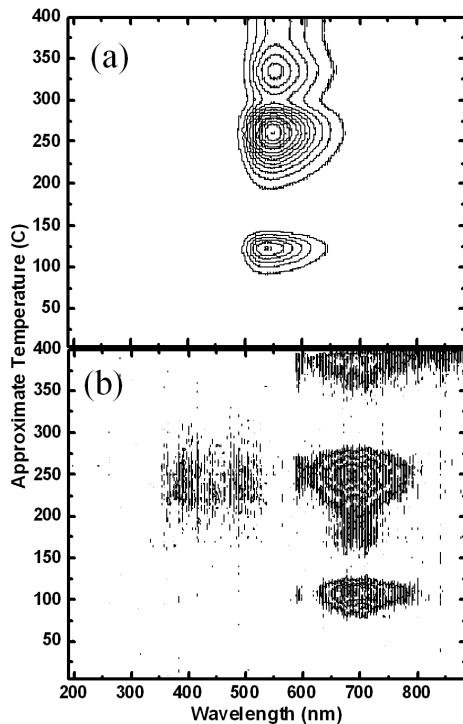
Fig. 2. Contour plot for the TL spectra shown in Fig. 1: (a) Ce doped YAG plotting luminescence intensity contours to a map of temperature versus wavelength. Each contour represents 1500 counts. (b) Undoped YAG, plotting luminescence intensity contours to a map of temperature versus wavelength. Each contour represents a step of 200 counts.
