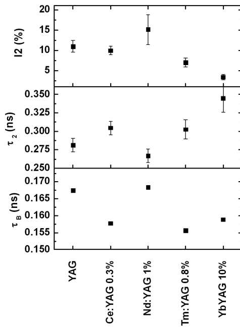
Fig. 3. Positron lifetime measurements in YAG single crystals grown in Ar atmosphere and doped with different rare earth metals. The graph shows the bulk lifetime, the defect lifetime and its intensity.
