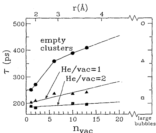
Fig.3. Calculated positron lifetimes in empty and He-filled 3-dimensional vacancy clusters (bubbles) in aluminum as functions of the number of vacancies in the cluster. "He/vac = 1 (or 2)" means that the number of He atoms in the cluster equals the number of vacancies (or is twice the number of vacancies). From [19].
