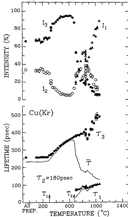
Fig.13 Positron lifetime parameters as functions of annealing temperature for Cu containing \sim 3 at % Kr. The longlived components are associated with Kr-bubbles ( \tau_3, I_3 ), and with small vacancy clusters containing Kr ( \tau_2, I_2 ). The lifetime \tau_3 is a measure of the Kr density in the bubbles. From [56].
