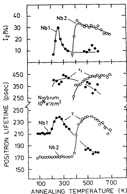
Fig.12. Annealing of electron irradiated pure ( \bullet ) and hydrogen containing ( \circ ) Nb. The average positron lifetime \bar{\tau} (Sec.4.1.) and the long-lived component \tau_2 , I_2 are shown as functions of annealing temperature. The appearance of the long-lived component at 220K (Nb1) is due to vacancy migration and clustering in pure Nb. For Nb2 the clustering is shifted to 380K due to hydrogen impurities. From [54].
