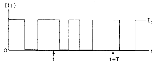
FIG. 2. Single-atom fluorescent intensity vs time. Interruptions of fluorescence are due to excitation of the weak transition 0 \rightarrow 2 .
