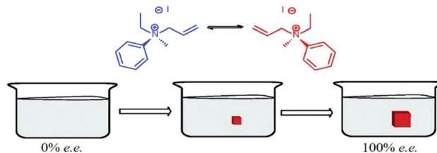
Fig. 13 Enantiomeric preferential crystallization of N,N,N -allylmethylanilinium iodide as described by Havinga. Fast racemization in solution supplies the growing crystal with the appropriate enantiomer. Adapted from ref. 55 with permission from the Royal Society of Chemistry, copyright 2015.
