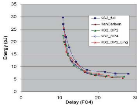
Fig. 14. KS and sparse variants
