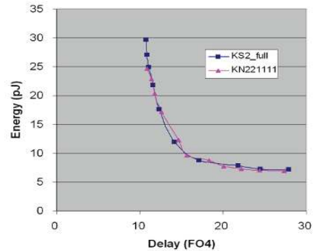
Fig. 13. KS vs. KN221111
