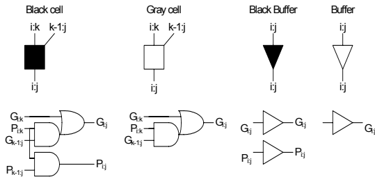
Fig. 2. Group GP cells
