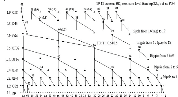
Fig. 10. Brent-Kung sparseness 4, with 10 levels (BK_L10)
