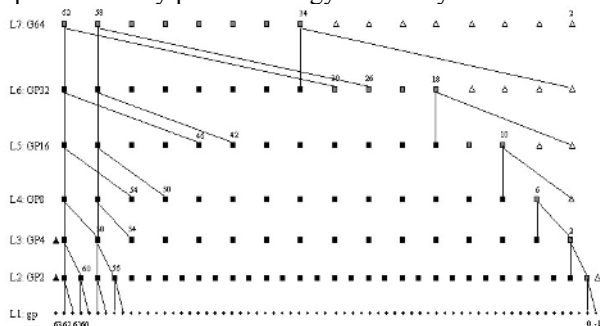
Fig. 4. Kogge-Stone sparseness 4
