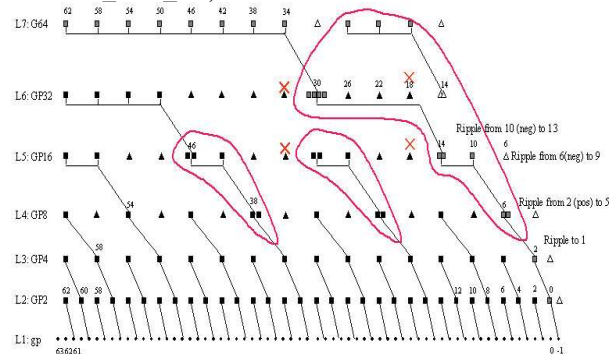
Fig. 8. New buffered sparse KN8421_FO2_LP (LP2)
