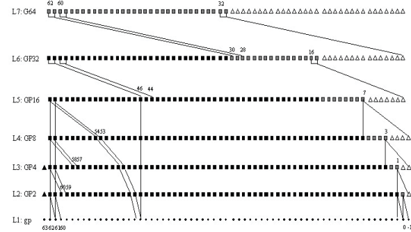
Fig. 3. Knowles [2,2,1,1,1,1]
