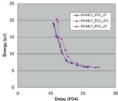
Fig. 15. KN8421 FO2 (both LP and LP2) & FO3
