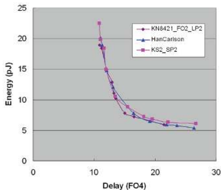
Fig. 16. FO2 vs. HC and SP2
