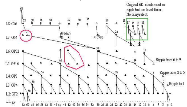
Fig. 11. Brent-Kung sparseness 4, with 9 levels (BK_L9)
