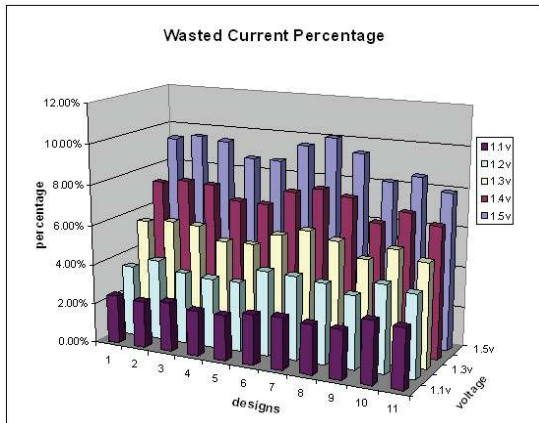
Fig. 19. Wasted current (short-circuit current) percentage (KN8421_FO2_LP2)
