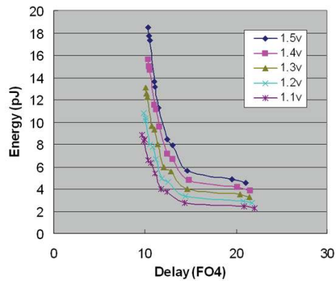
Fig. 18. VDD Scaling (KN8421_FO2_LP2) (FO4 inverter delay is 51ps, 55ps, 61ps, 68ps and 79ps for VDD 1.5v, 1.4v, 1.3v, 1.2v and 1.1v, respectively) (a) Delay in picoseconds (b) Delay in fanout-of-four inverter delay
