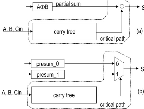
Fig. 1. General structures of two types of CLA adders (a) pure CLA without carry select (b) Hybrid sparse CLA with carry select
