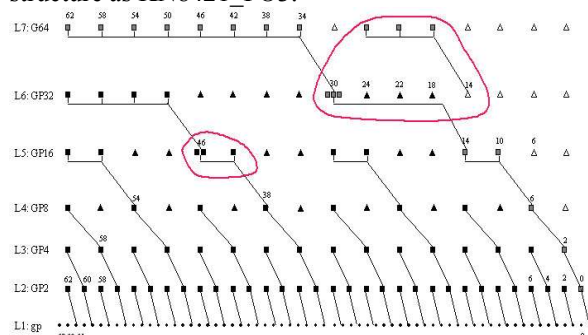
Fig. 7. New buffered sparse KN8421_FO3
