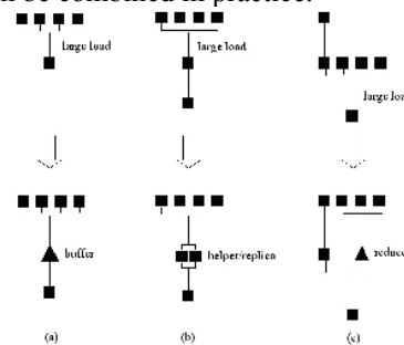
Fig. 6. Buffering: (a) normal (b) helper/replica (c) reducer
