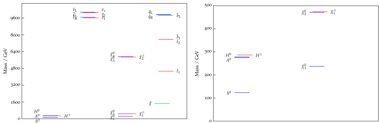
FIG. 4 (color online). Left: Full spectrum of the NUHM2 benchmark. Right: Zoom into the spectrum below 500 GeV.
