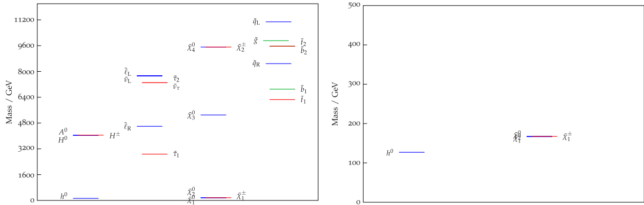
FIG. 9 (color online). Left: Full spectrum of the BB benchmark. Right: Zoom into the spectrum below 500 GeV.
