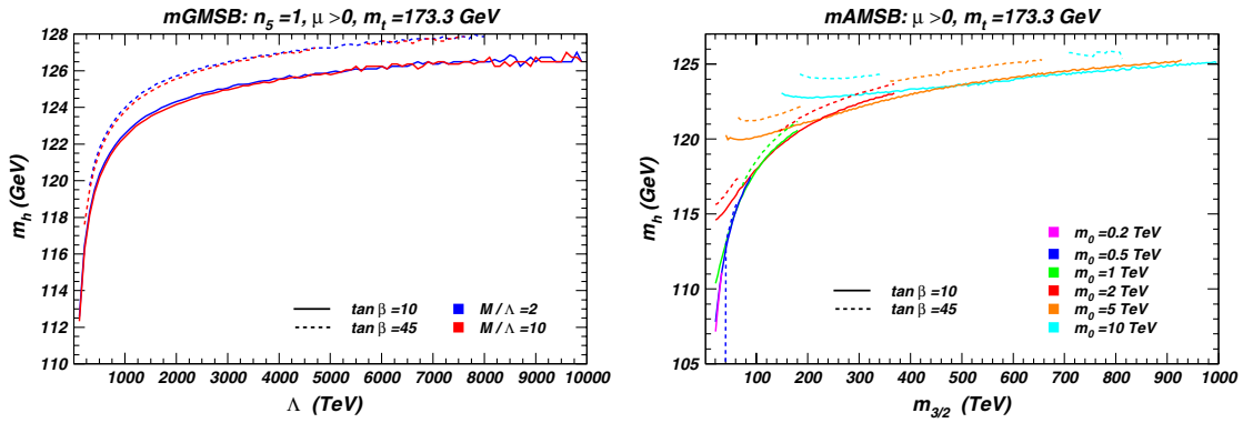
FIG. 1 (color online). Value of m_h in mGMSB and in mAMSB versus \Lambda and m_{3/2} from [40].
