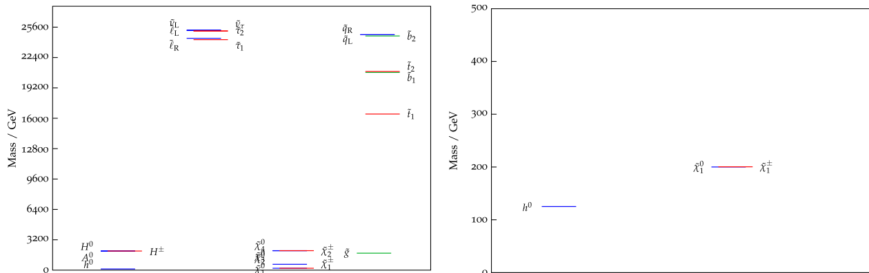
FIG. 8 (color online). Left: Full spectrum of the KL benchmark. Right: Zoom into the spectrum below 500 GeV.
