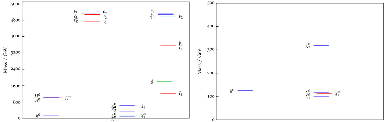
FIG. 3 (color online). Left: Full spectrum of the RNS benchmark. Right: Zoom into the spectrum below 500 GeV.
