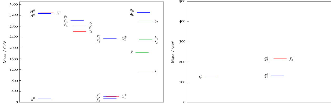
FIG. 6 (color online). Left: Full spectrum of the NUGM benchmark. Right: Zoom into the spectrum below 500 GeV.
