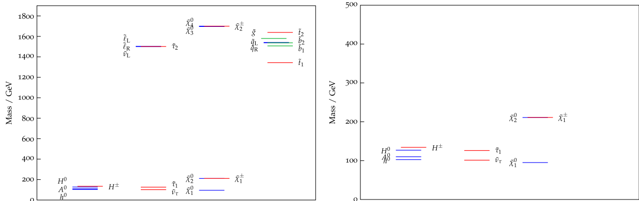
FIG. 11 (color online). Left: Full spectrum of the low MH benchmark. Right: Zoom into the spectrum below 500 GeV.
