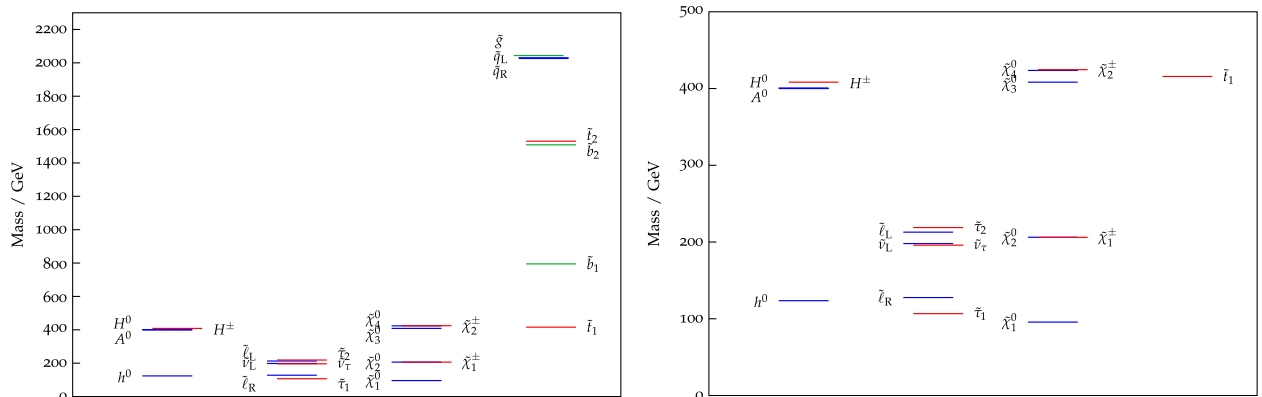
FIG. 7 (color online). Left: Full spectrum of the STC benchmark. Right: Zoom into the spectrum below 500 GeV.
