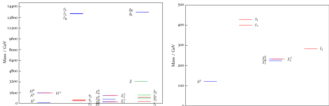
FIG. 2 (color online). Left: Full spectrum of the natural SUSY benchmark. Right: Zoom into the spectrum below 500 GeV.
