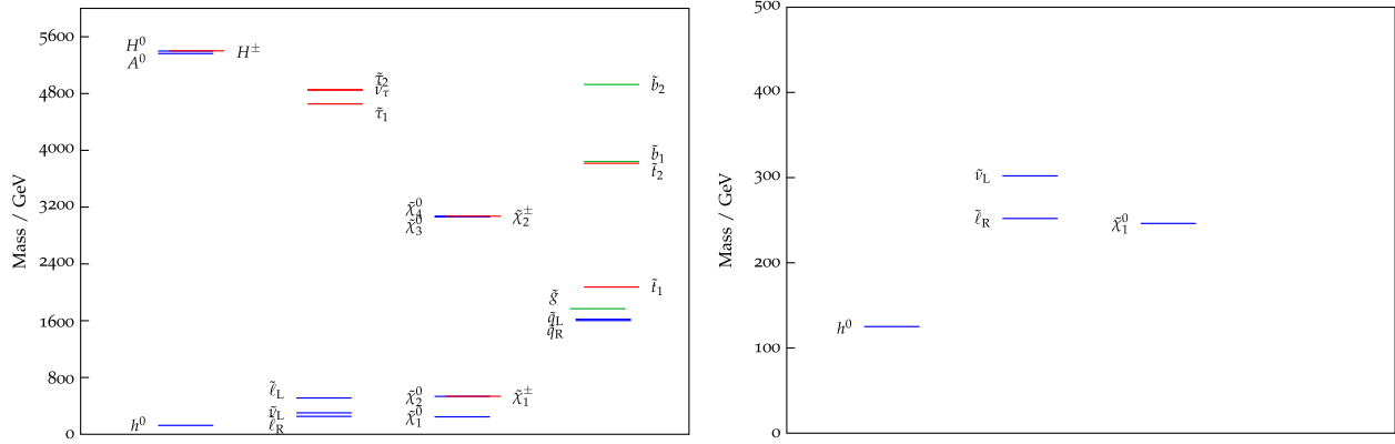
FIG. 10 (color online). Left: Full spectrum of the NMH benchmark. Right: Zoom into the spectrum below 500 GeV.
