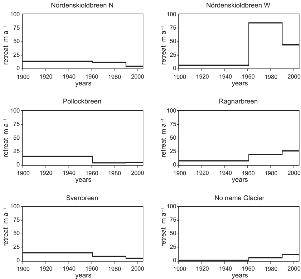
Fig. 8. Linear mean retreat rates of glaciers in Billefjorden region for following periods: 1900–1961, 1961–1990 and 1990–2002 (continued).
