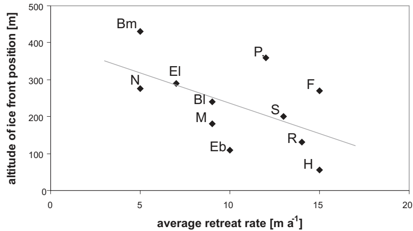
Fig. 11. Relation of average retreat rate (for the last decade) and elevation of the ice front positions (Bl – Bertil; Bm – Bertram; Eb – Ebba; El – Elsa; F – Ferdinand; H – Hørbye; M – McWhae; N – No name; P – Pollock; R – Ragnar; S – Sven; Nordenskiöldbreen not included).
