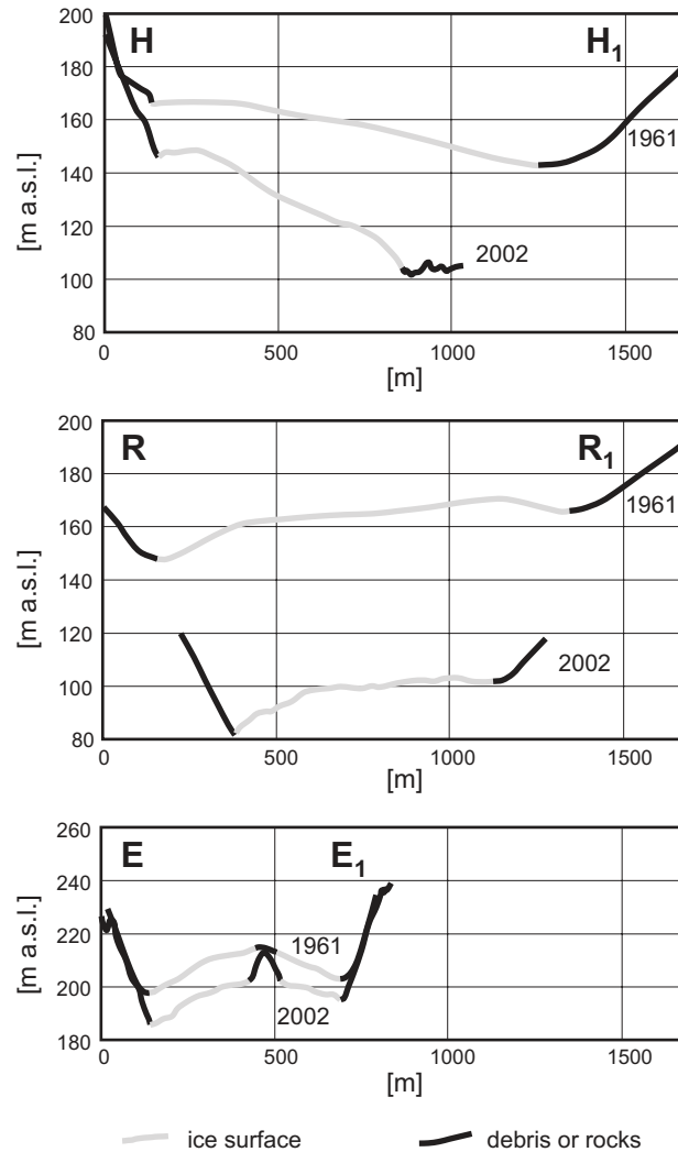
Fig. 10. Changes in ice thickness of Ebbabreen, Hørbreen and Ragnarbreen between 1961 and 2002. Locations of the transects are marked on Fig. 1.
