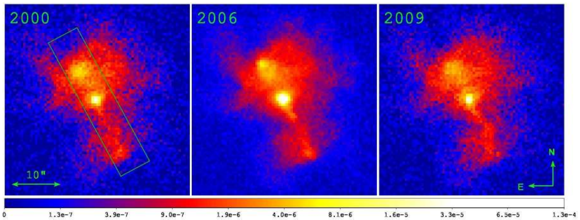
FIG. 6.— Exposure-corrected Chandra ACIS images of the PWN associated with PSR J1846–0258 in 1 – 7 keV. The 6'' wide box along a position angle of 27^\circ (North through East) is analyzed in detail for each epoch in Figure 7.
