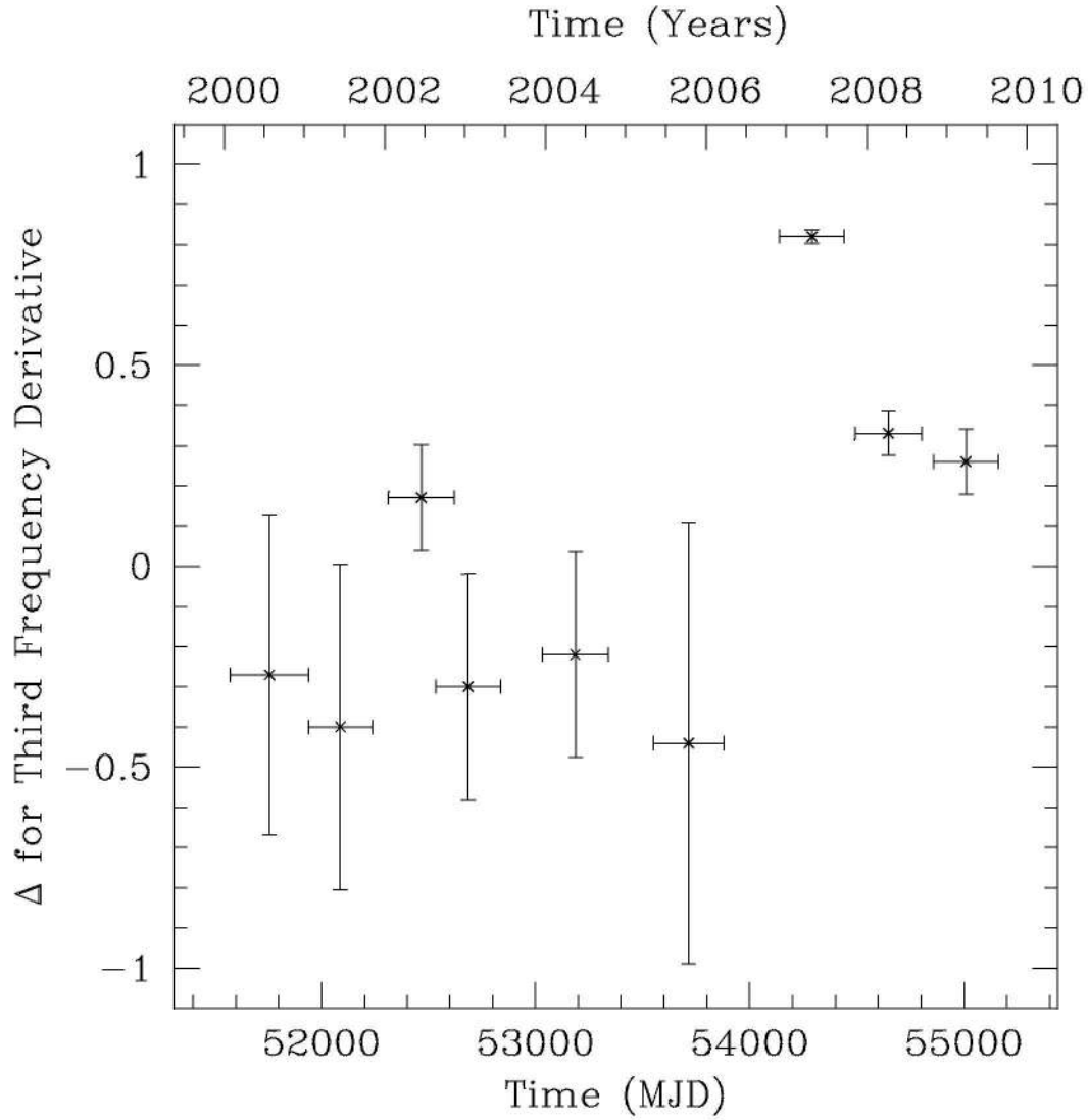
FIG. 5.— A quantification of the timing noise in PSR J1846–0258 over 10 yr. Each point is a measurement of the \Delta_{\dot{\nu}} parameter for approximately 2.5 \times 10^7 s. This provides an estimate of the amount of timing noise observed in the pulsar, and shows a dramatic increase after the large glitch observed in 2006.
