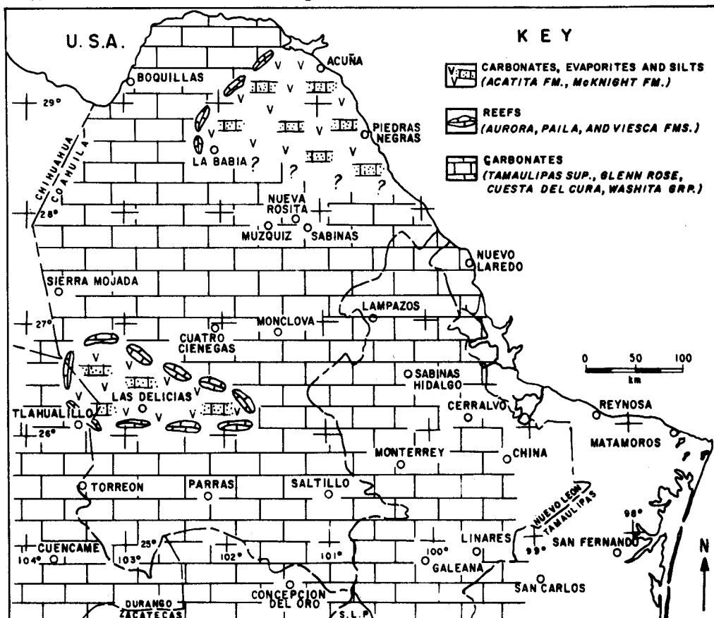
Fig. 9. Albian - Cenomanian paleogeography of northeast Mexico.
