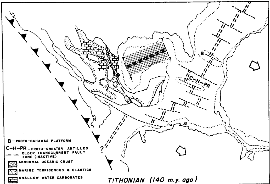
Fig. 26. Paleo-reconstruction at 140 Ma.
