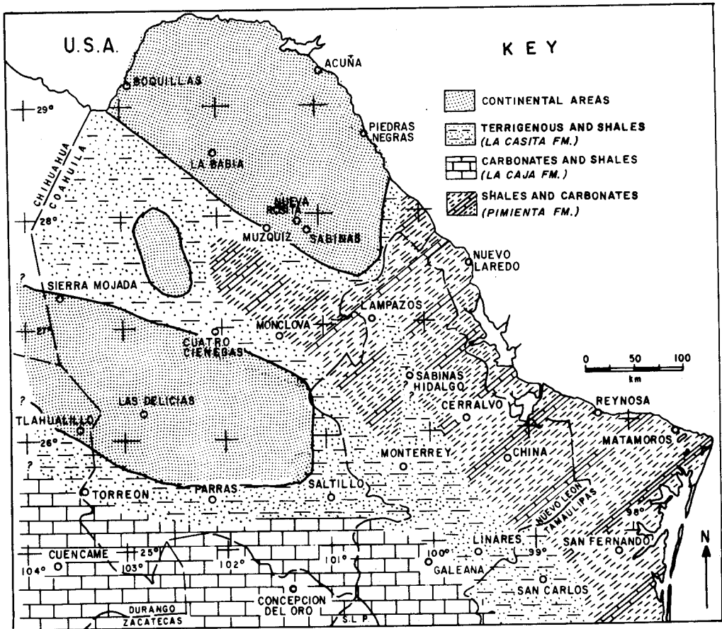
Fig. 6. Late Kimmeridgian - Tithonian paleogeography of northeast Mexico.
