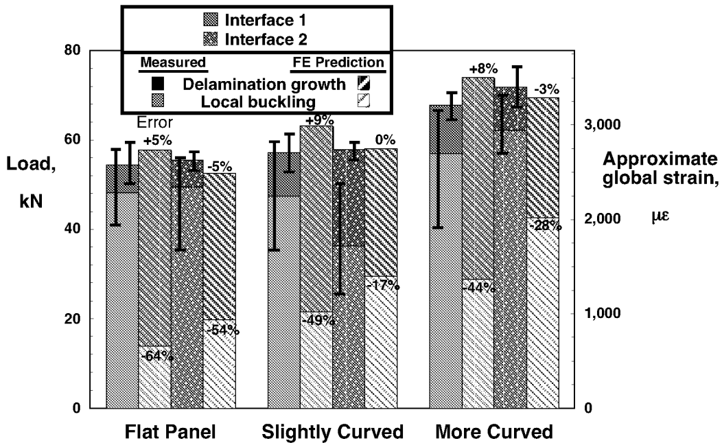
Figure 8. Comparison of experimental and analytical results for sublaminates buckling and delamination growth.
