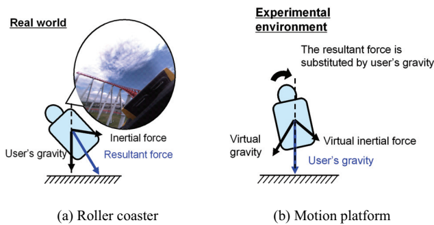
Figure 2: Realization of inertial force sensation
