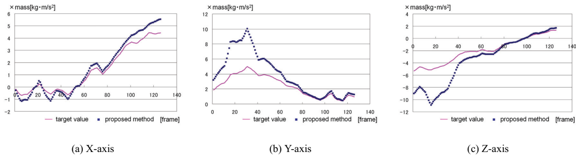
Figure 4: Result of estimated inertial force
