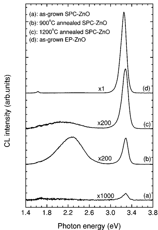
FIG. 5. Cathodoluminescence spectra obtained for the as-grown and annealed SPC-ZnO and as-grown EP-ZnO.
